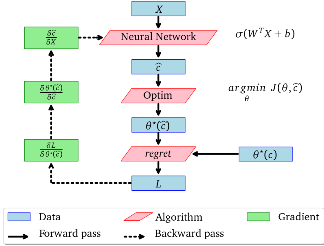
Figure 2.16 – In Decision-Focused Learning , the regret is taken into account during the training of the Neural Network that forecasts \hat{c} . The chain rule is applied and the gradient of the solution to the optimization problem with respect to its input \frac{\partial \theta^*(\hat{c})}{\partial \hat{c}} has to be estimated.
