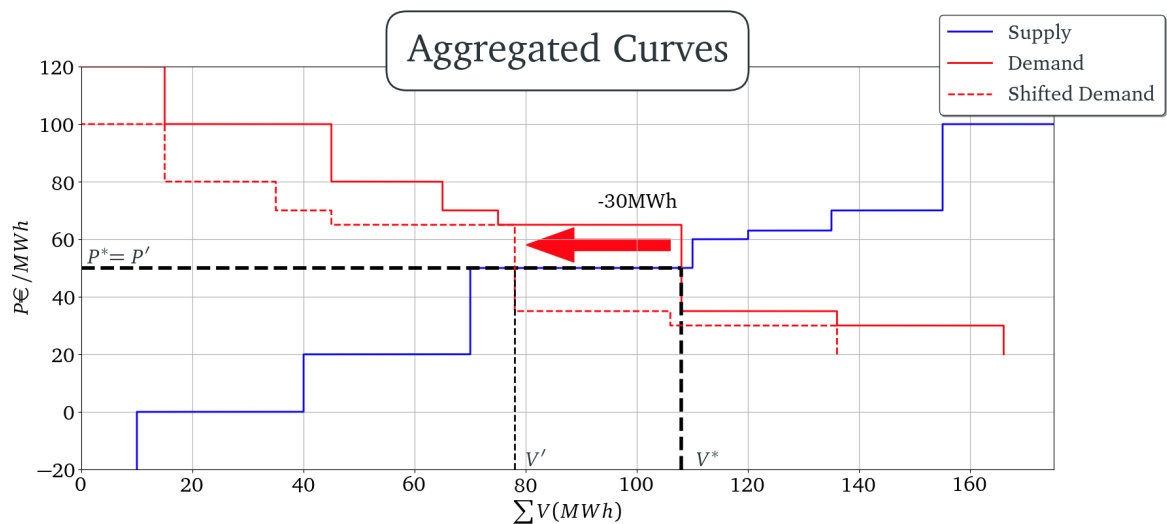
Figure 2.9 – Arbitrary Aggregated Curves with the supply in blue and demand in red. A medium shift of 30MWh in demand (red-dashed line) does not change the optimal price P^*
